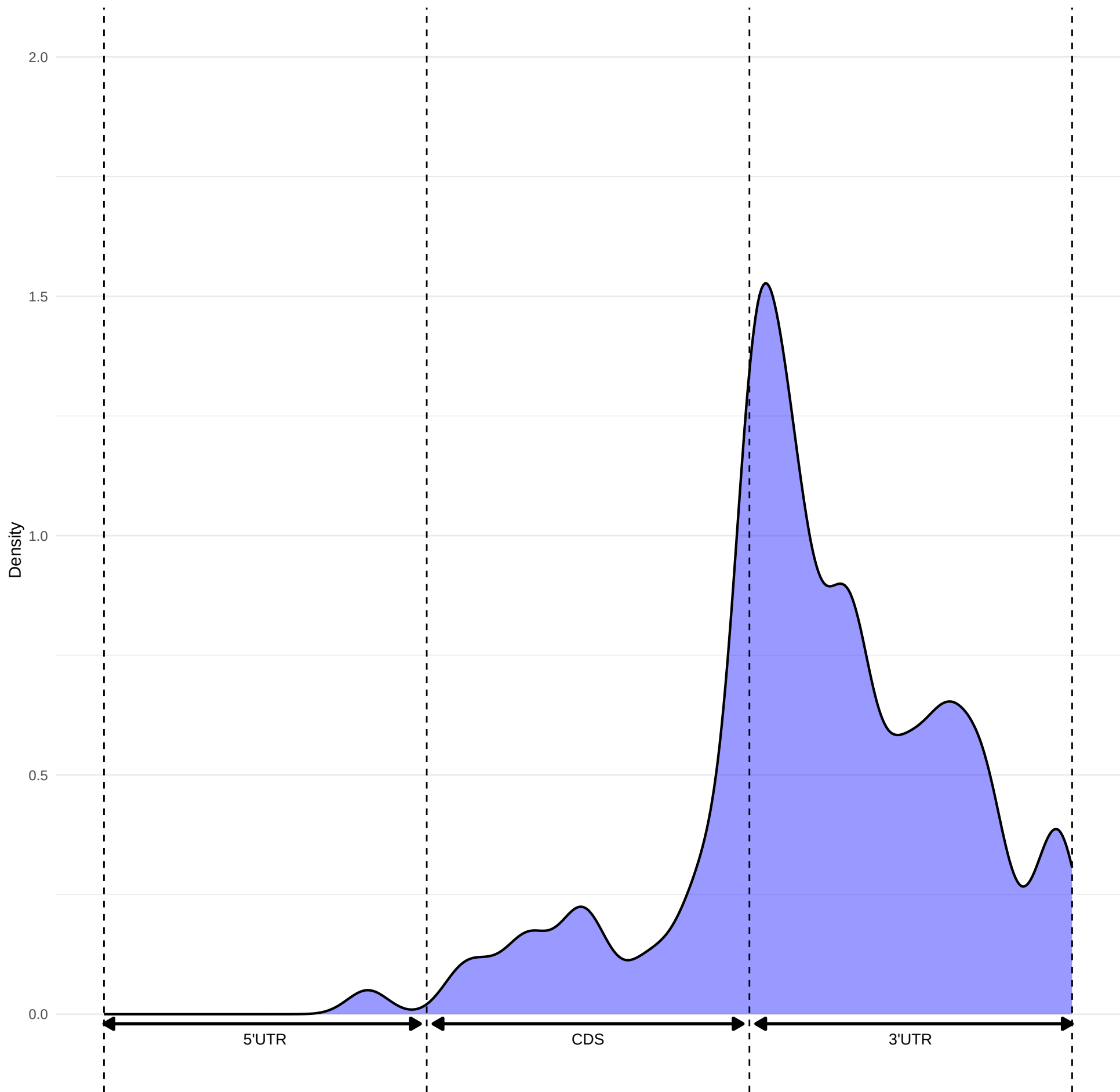
Transcriptome-wide m6A Distribution for: igf2bp2_kd
