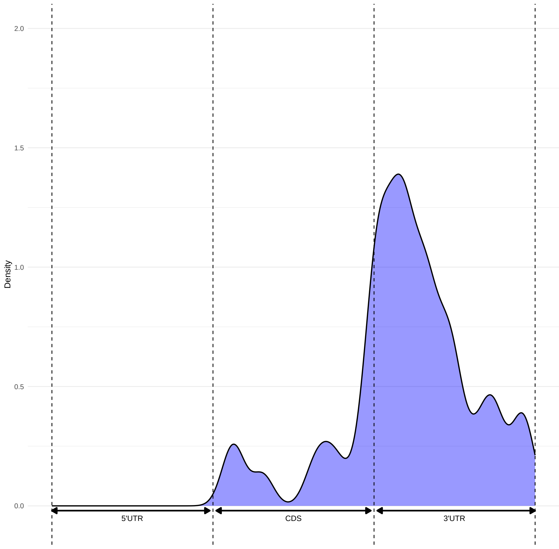
Transcriptome-wide m6A Distribution for: alkbh5_kd
