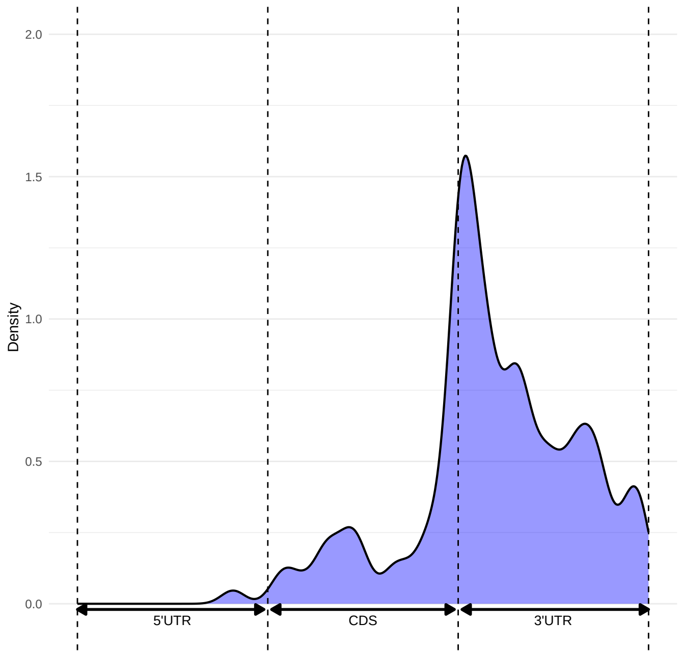
Transcriptome-wide m6A Distribution for: naive
