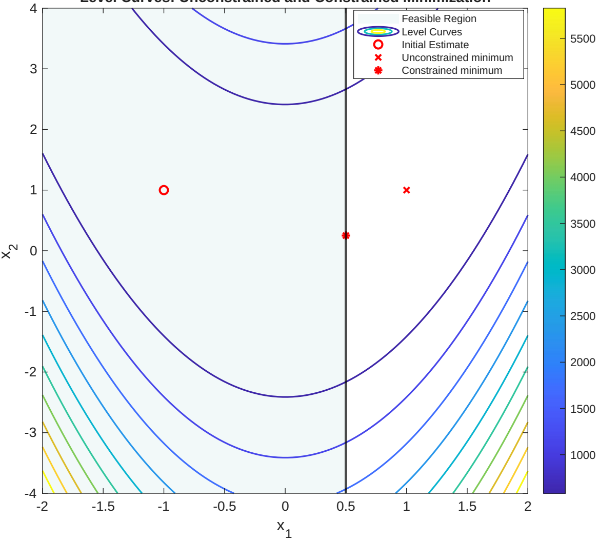
Level Curves: Unconstrained and Constrained Minimization
