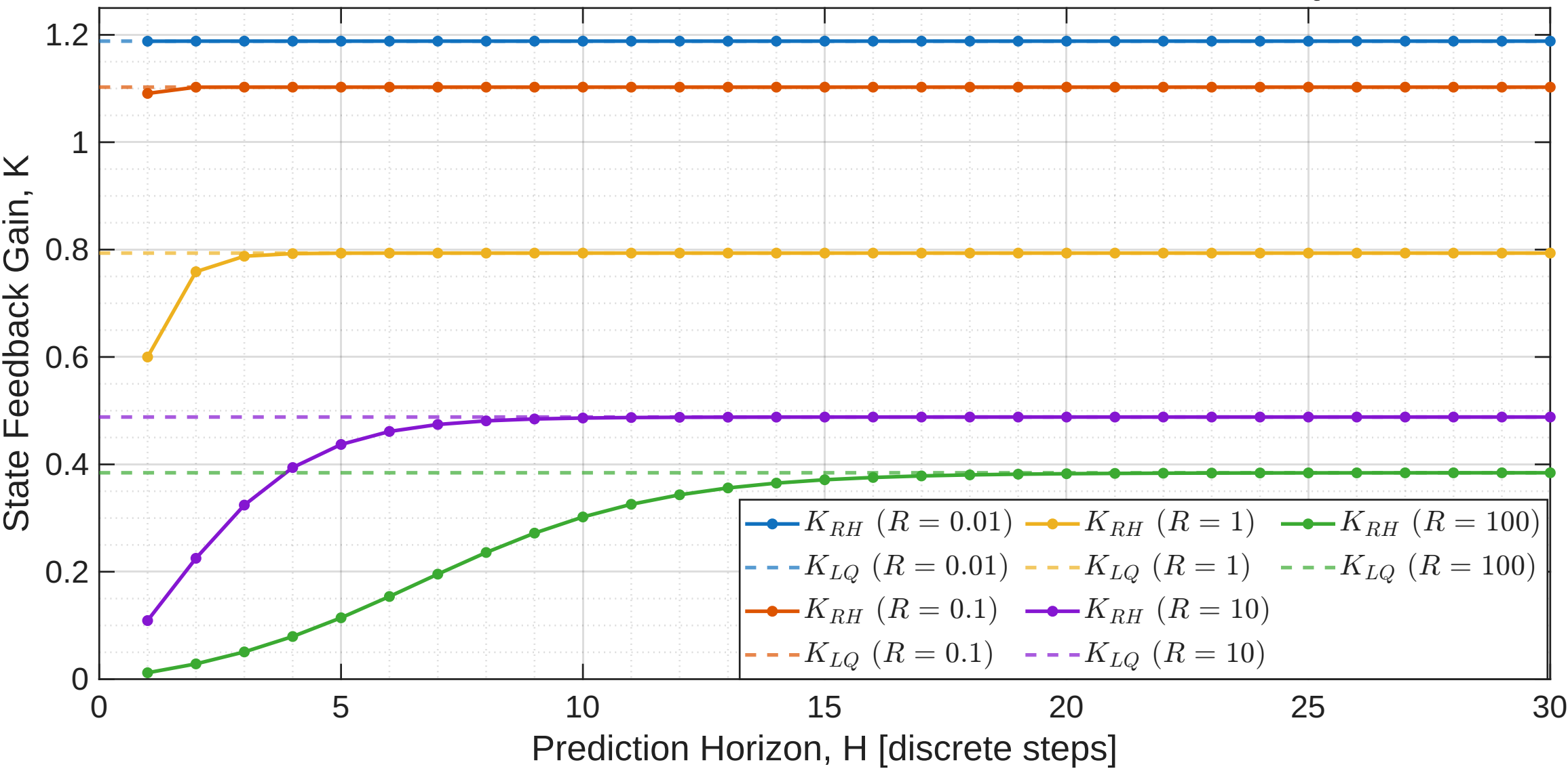
Asymptotic Convergence of Receding-Horizon Gain K_{RH} towards K_{LQ}
