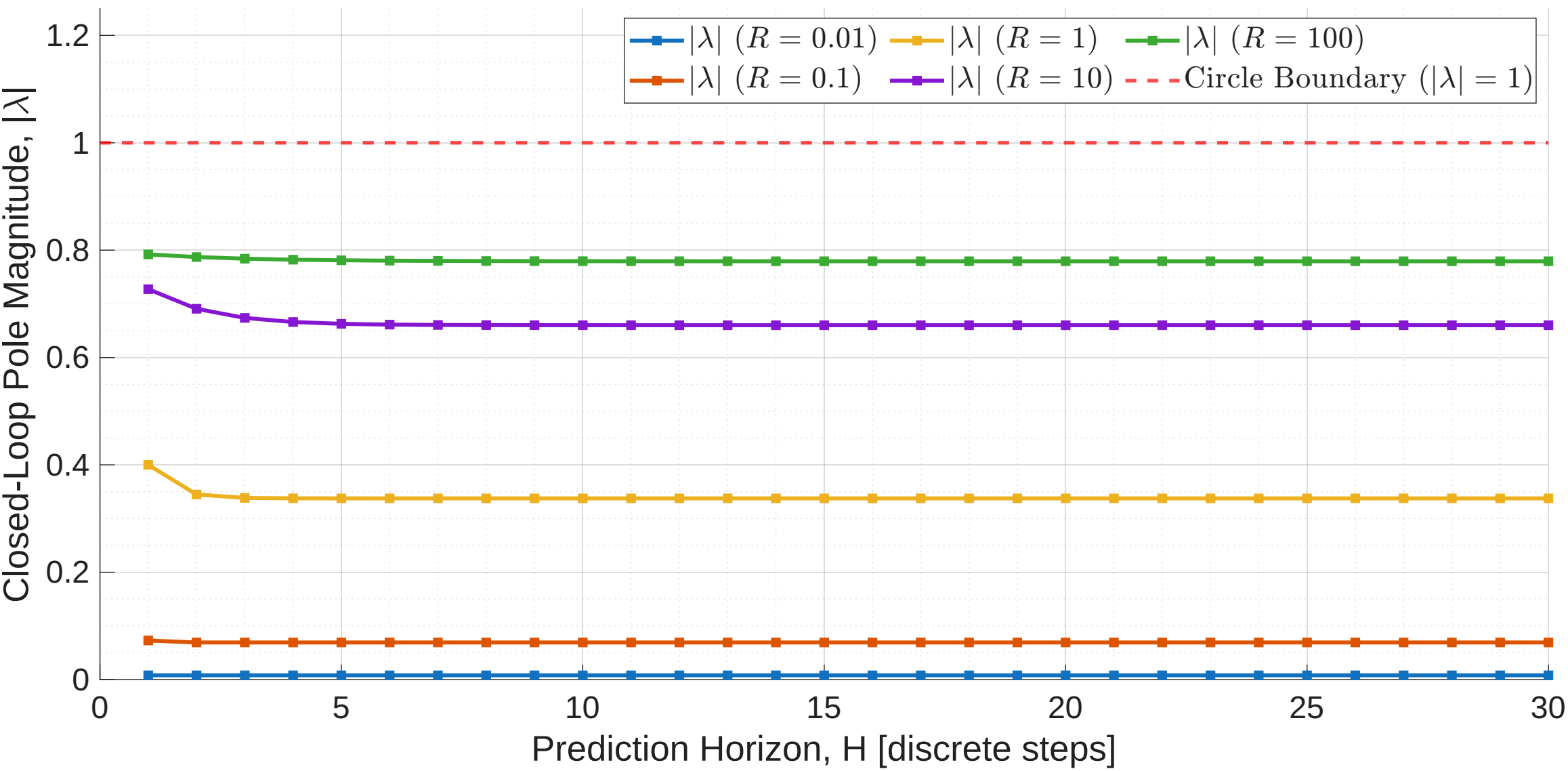
Closed-Loop Pole Modulus |\lambda| as a Function of Horizon H
