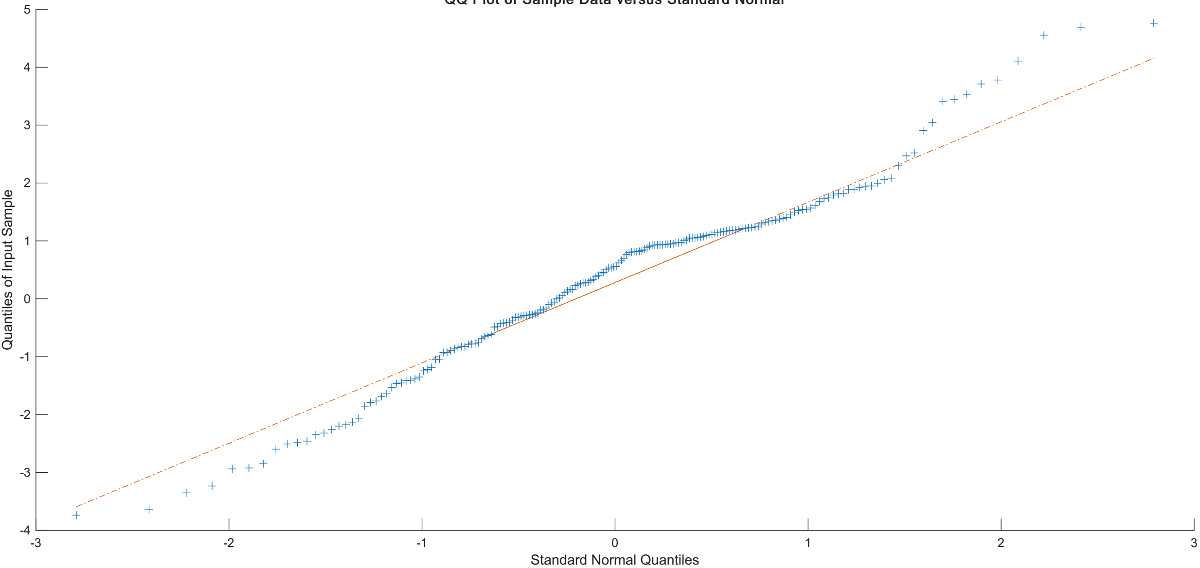
QQ Plot of Sample Data versus Standard Normal
