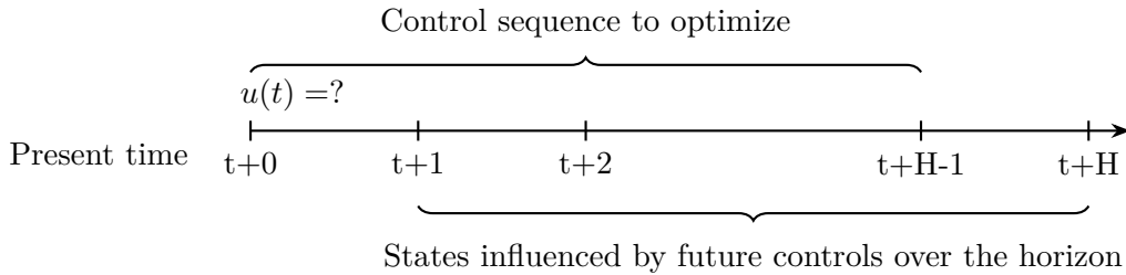
Figure 2: The control sequence to optimize in the receding-horizon cost and the corresponding sequence of states that is influenced by it.
