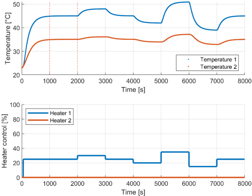
Figure 3: Simulated example of experiment for model identification.
