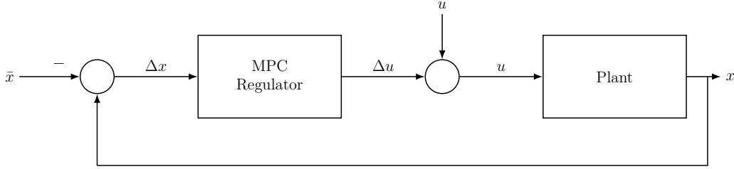
Figure 5: Illustration of the MPC regulator of incremental variables and feedforward control.
