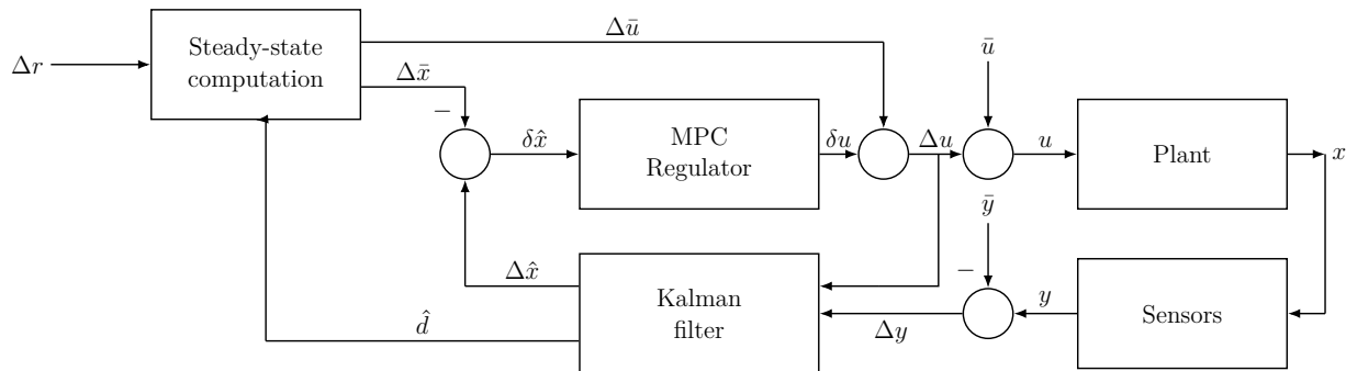
Figure 7: Illustration of the zero-offset MPC tracker with feedforward control and Kalman filter.
