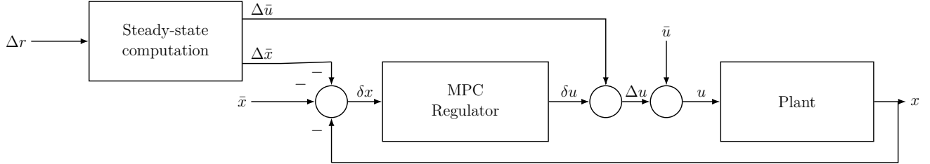
Figure 6: Illustration of the MPC tracker with feedforward control.
