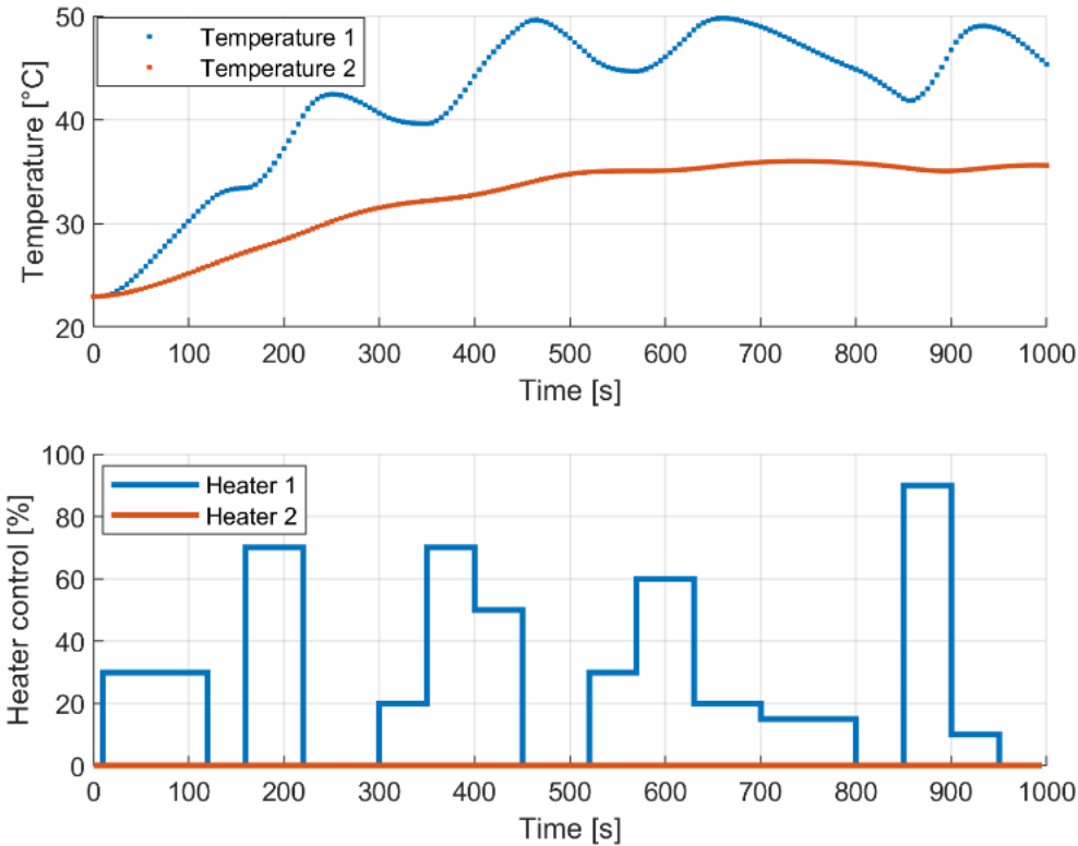
Figure 4: Simulated example of experiment for model validation.
