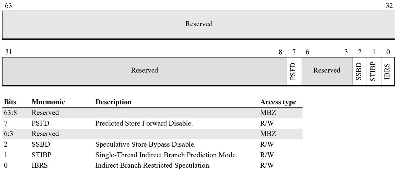
Figure 3-13. SPEC_CTRL Register
