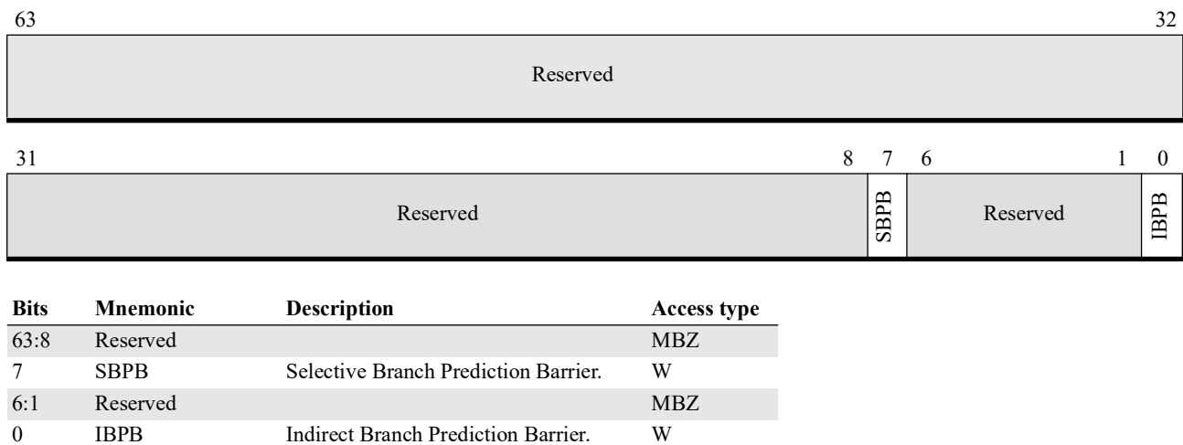
Figure 3-14. PRED_CMD Register
