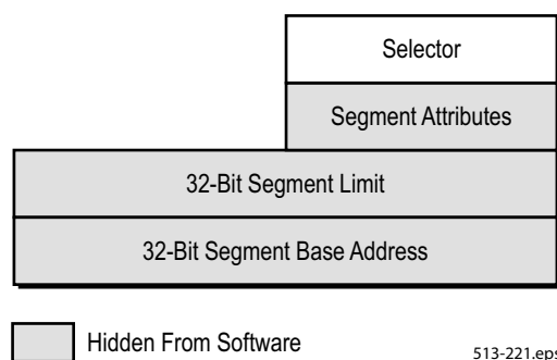
Figure 4-4. Segment-Register Format
