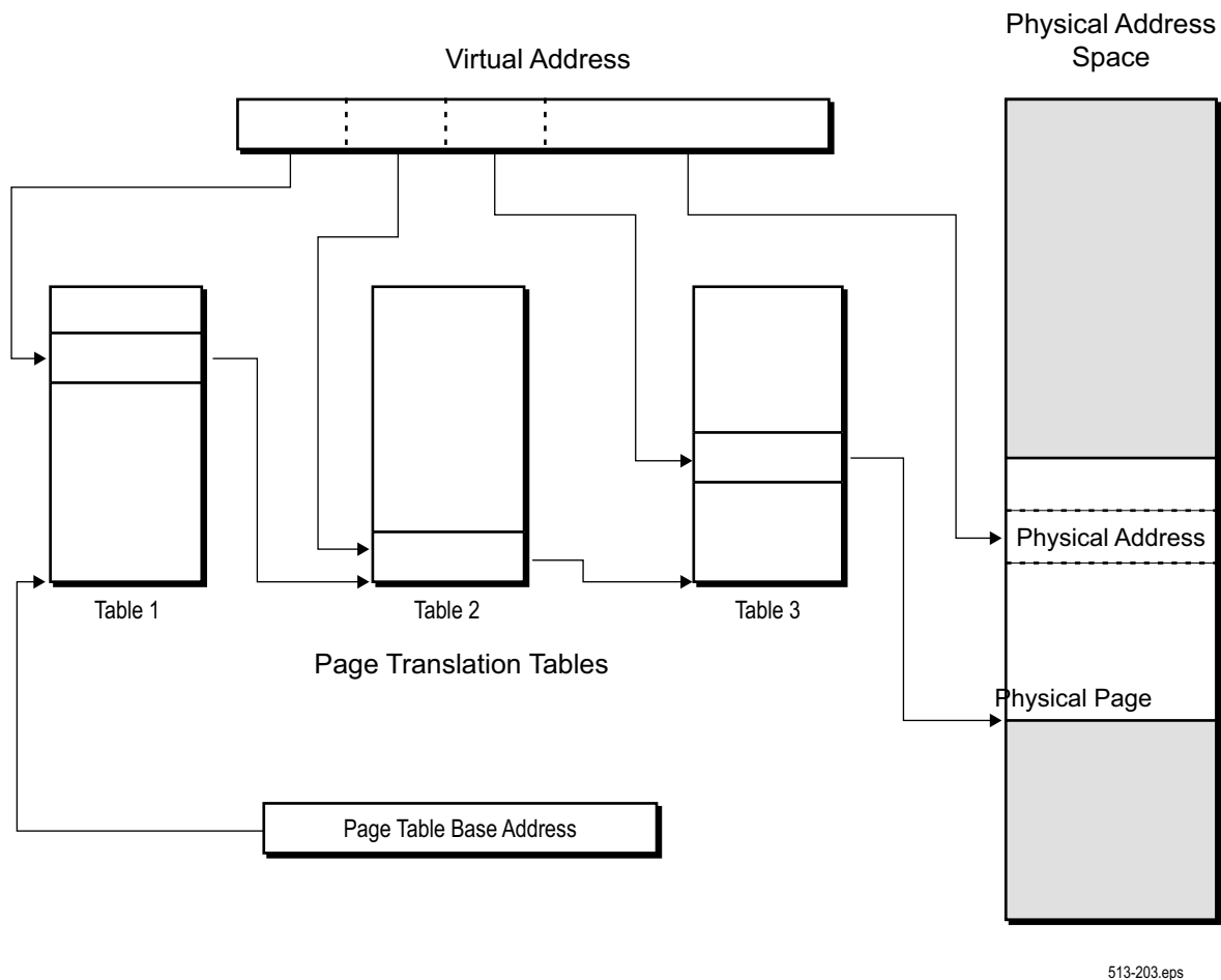
Figure 1-3. Paged Memory Model
