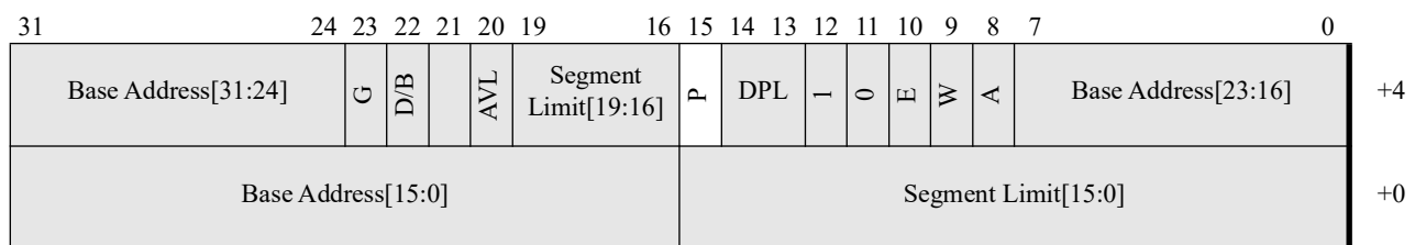
Figure 4-21. Data-Segment Descriptor—Long Mode
