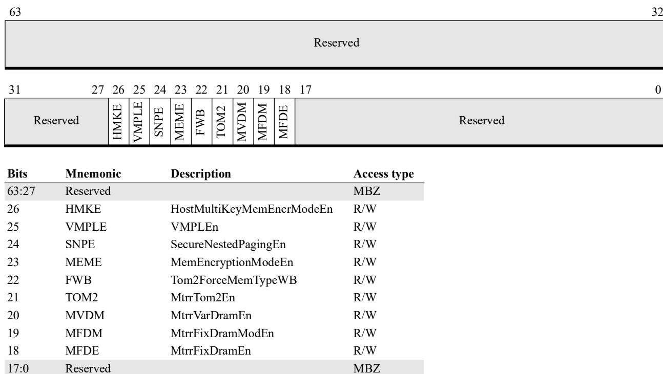
Figure 3-11. System-Configuration Register (SYSCFG)
