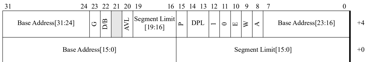
Figure 4-15. Data-Segment Descriptor—Legacy Mode
