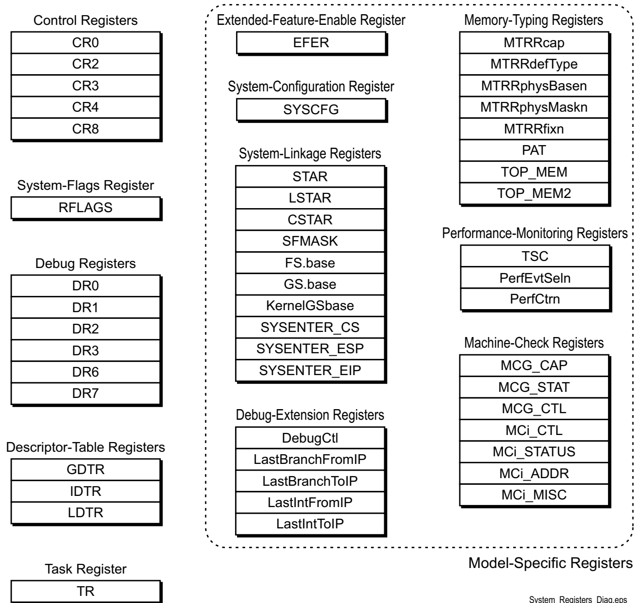
Figure 1-7. System Registers
