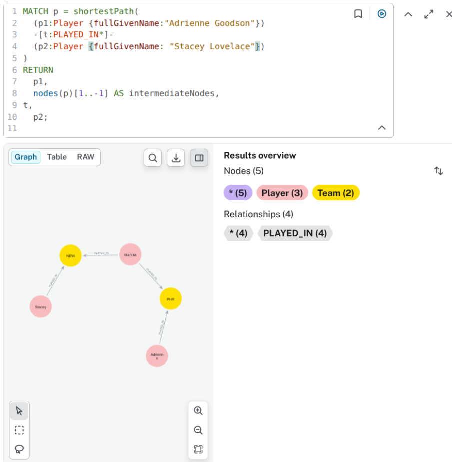
Figure 17: Shortest path between the two players.
