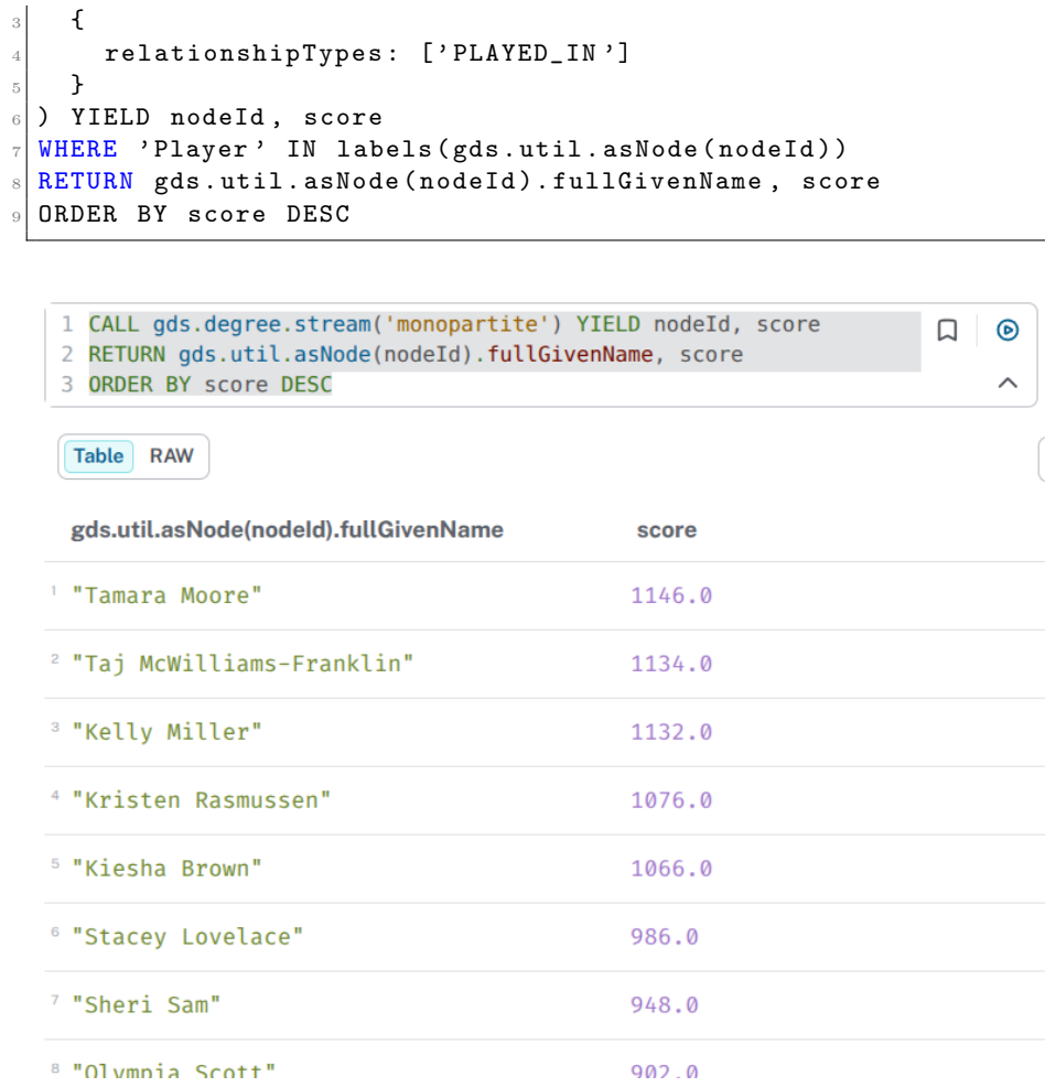
Figure 16: Most central players in the monopartite graph.
