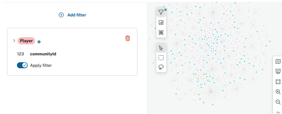
Figure 12: Detecting communities
