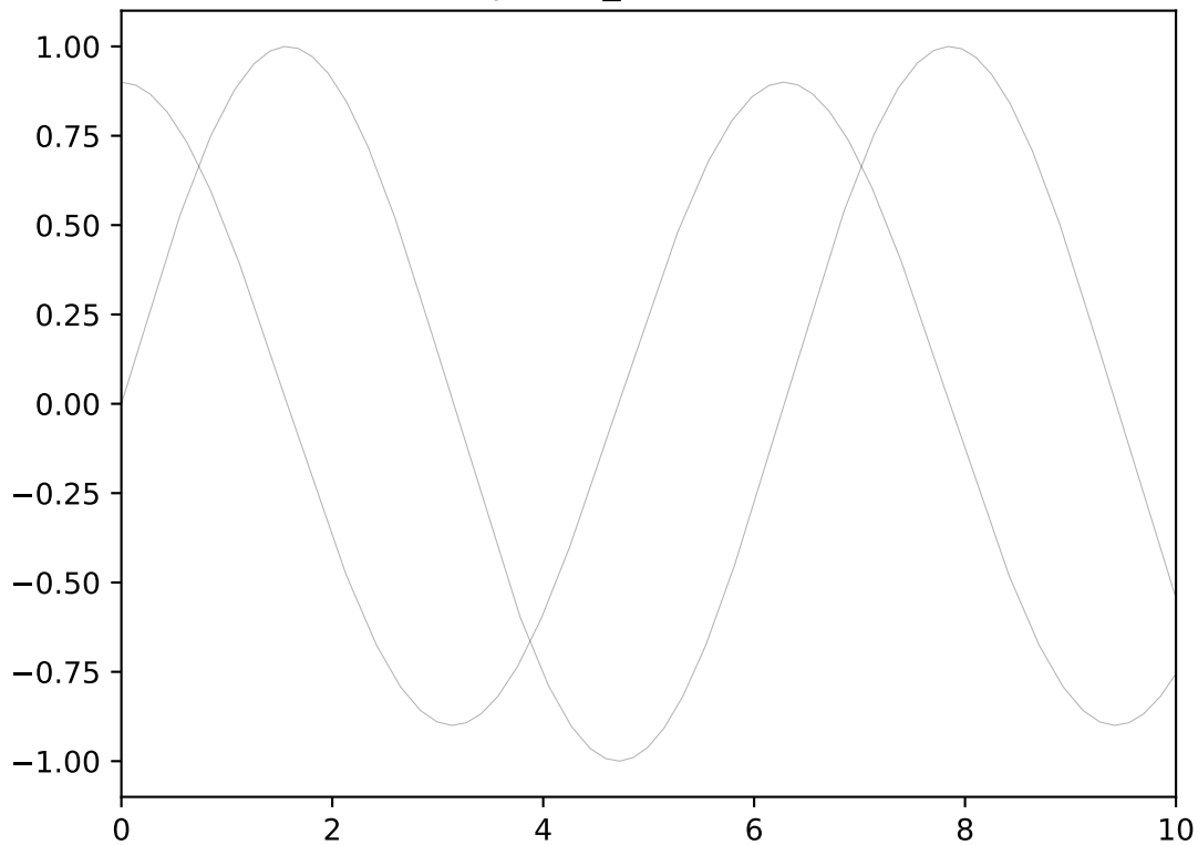
interpolate_cross (thr=1.0)
