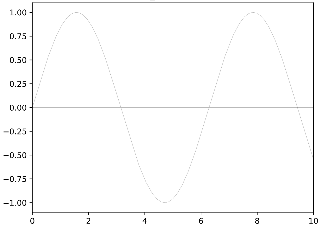
where_even (thr=1.0)
