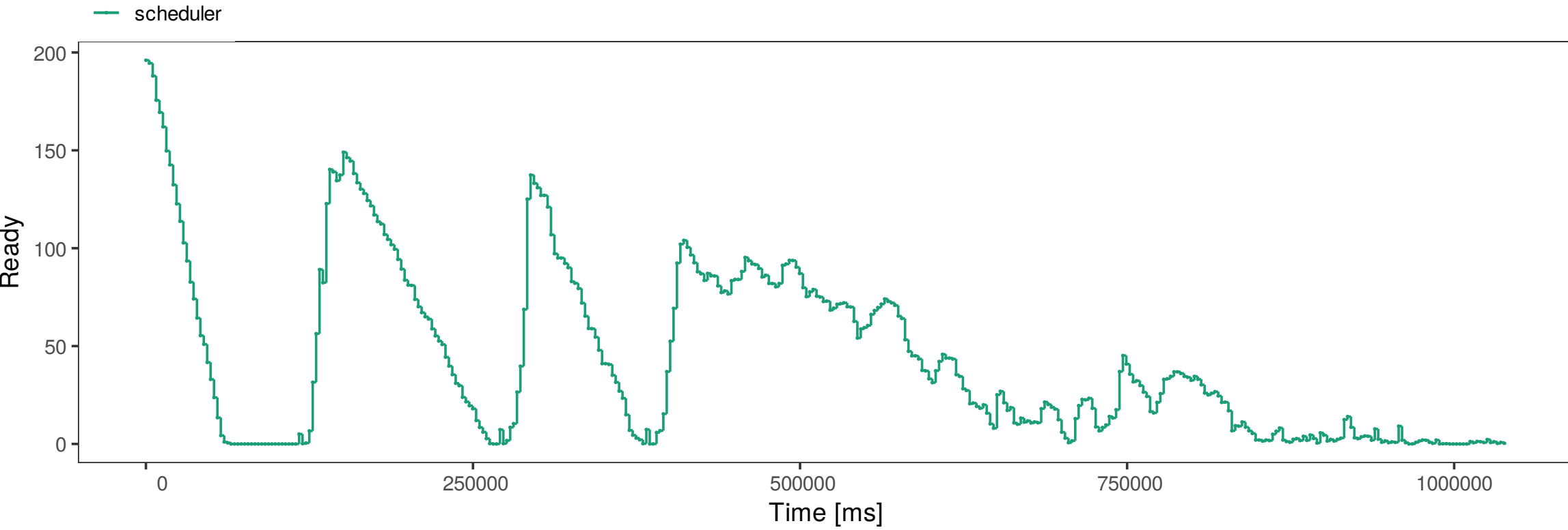
panel_ready (StarVZ) -- PaRSEC lfq spotrf n19200 b960
