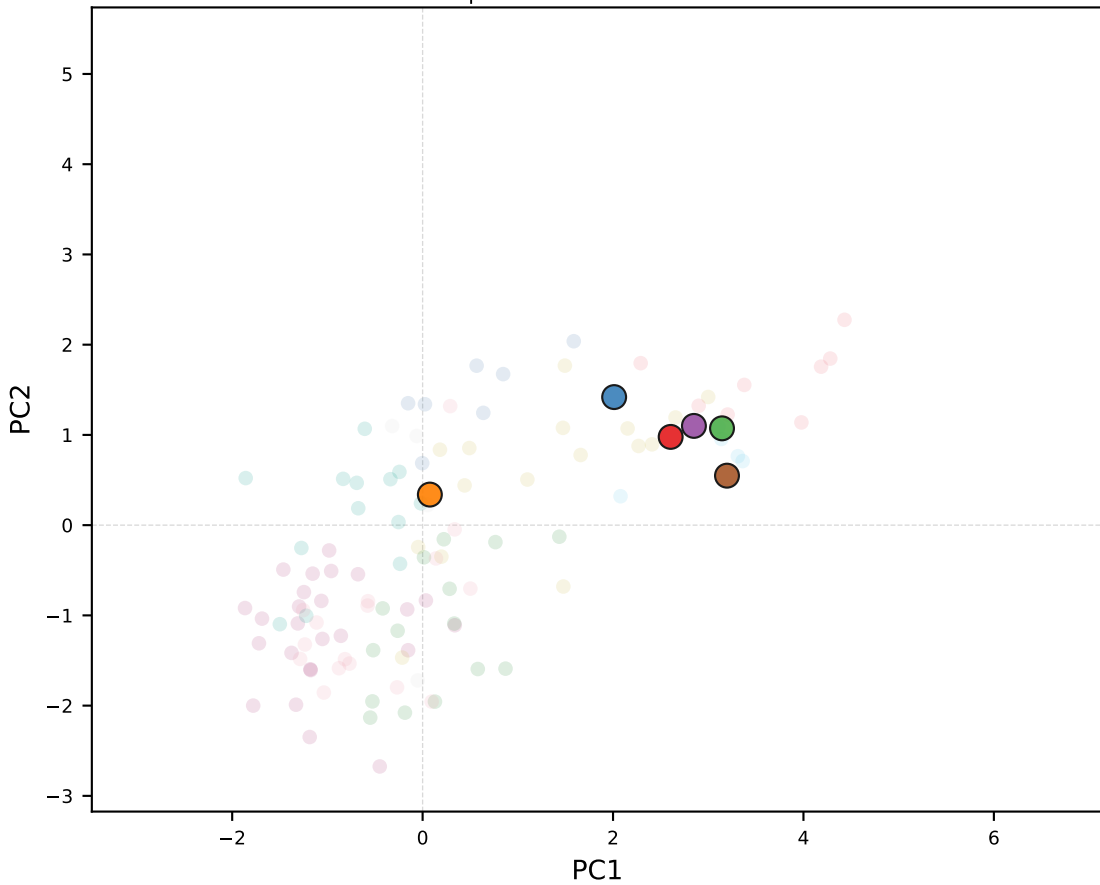
phi-3-mini-128k-instruct
