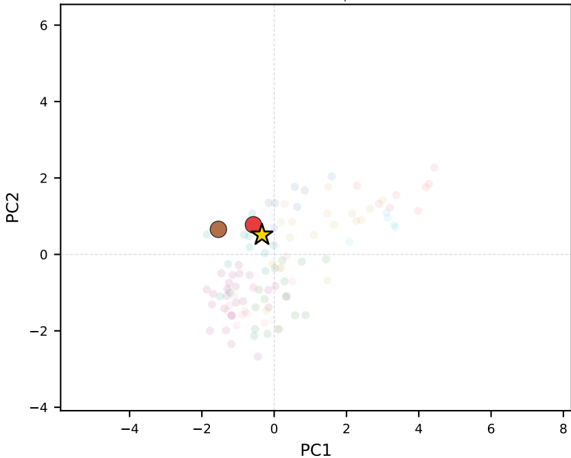
claude-sonnet-4.5 | Belarus
