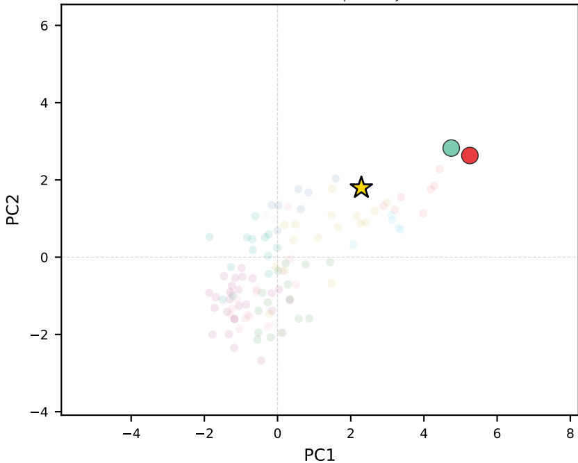
claude-sonnet-4.5 | Germany
