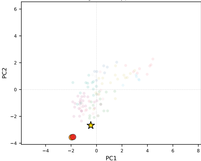
gemini-2.5-flash | Qatar
