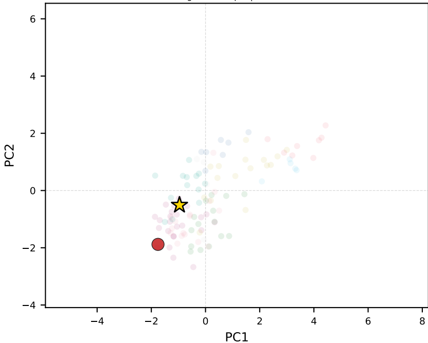
gemini-2.5-pro | Zambia
