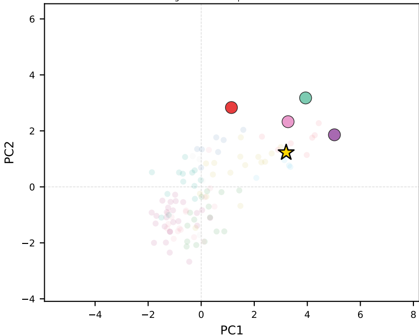
gemma-3-4b-it | Switzerland
