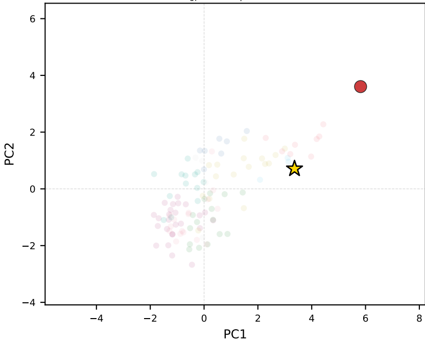
gpt-4o-mini | Australia
