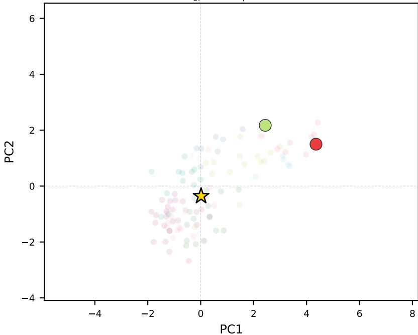
gpt-4o-mini | Brazil
