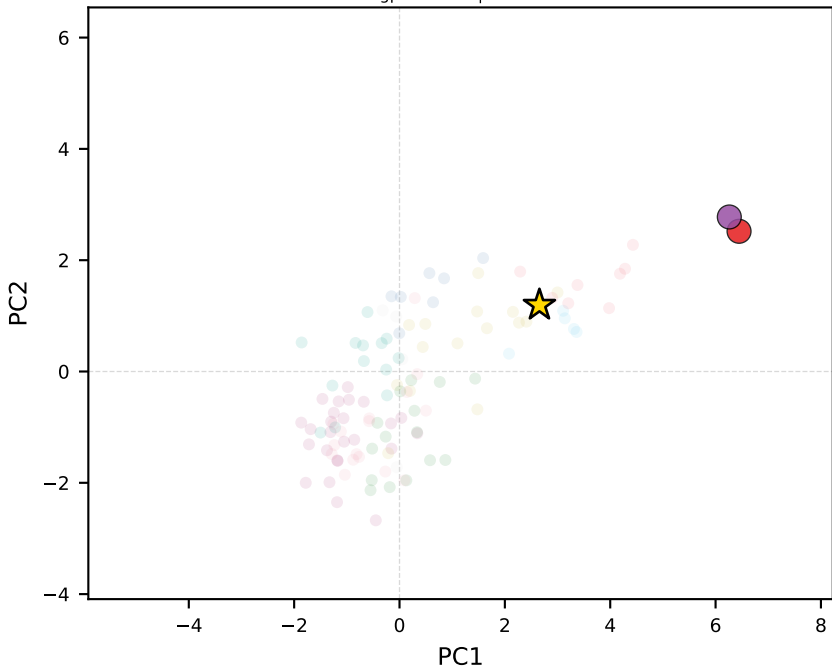
gpt-4o-mini | France
