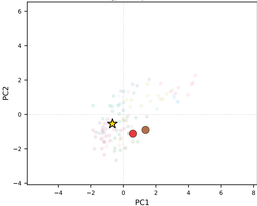
gpt-4o-mini | Kazakhstan
