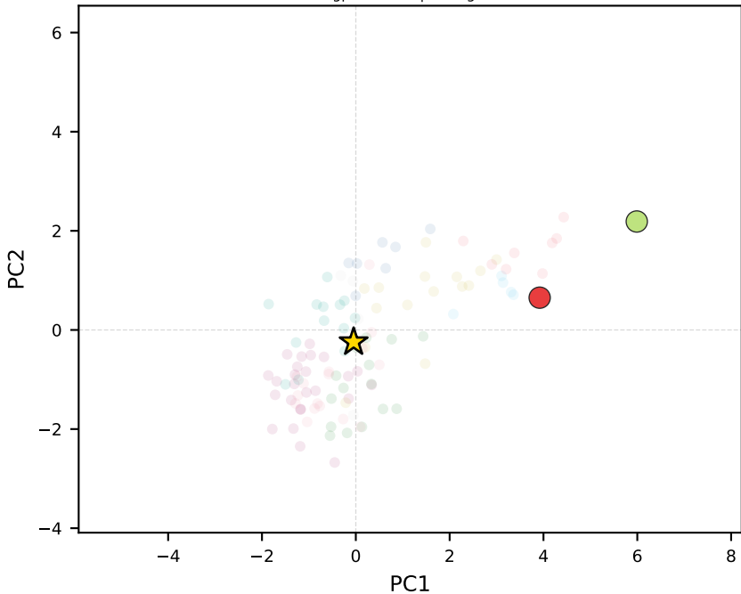
gpt-4o-mini | Portugal
