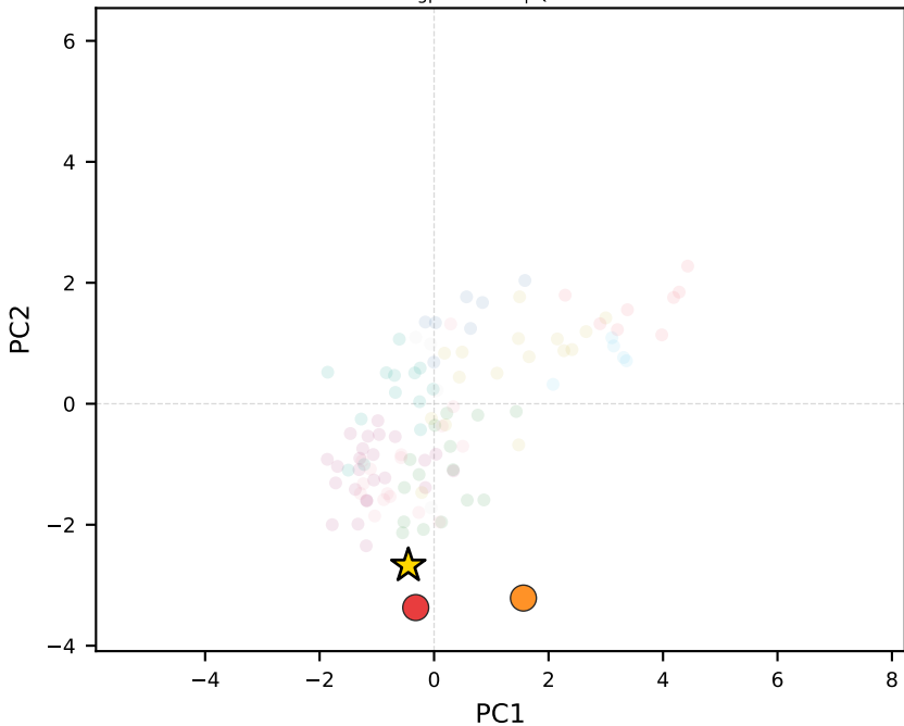
gpt-4o-mini | Qatar
