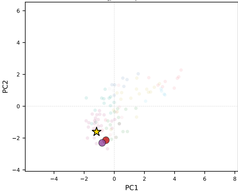
gpt-4o-mini | Rwanda
