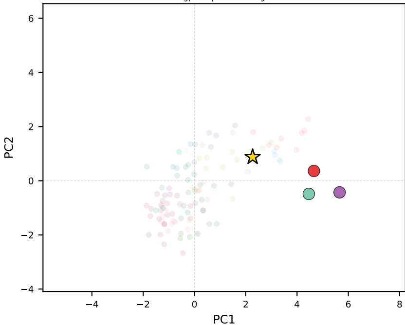
gpt-4o | Luxembourg
