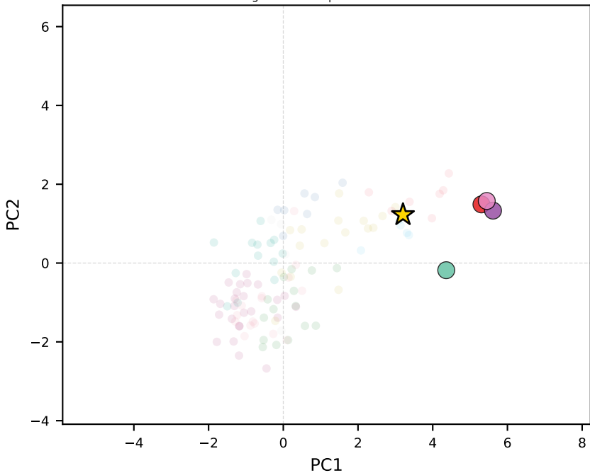
grok-4.1-fast | Switzerland
