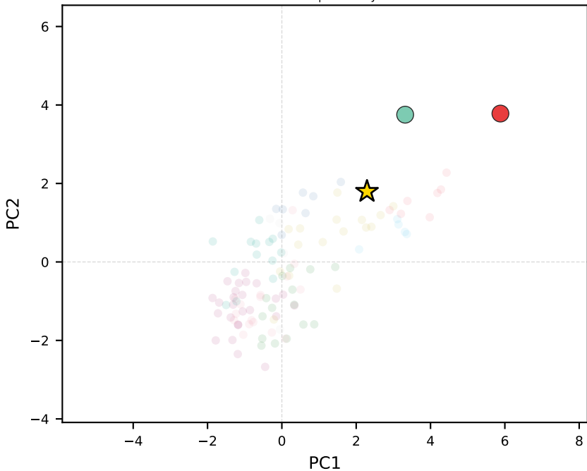
kimi-k2 | Germany
