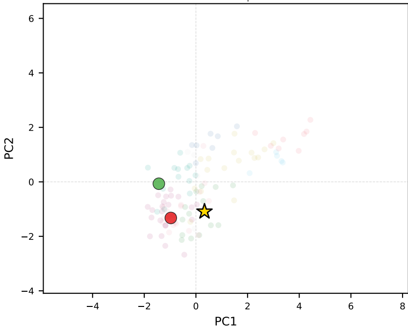
llama-3.3-70b-instruct | Guatemala
