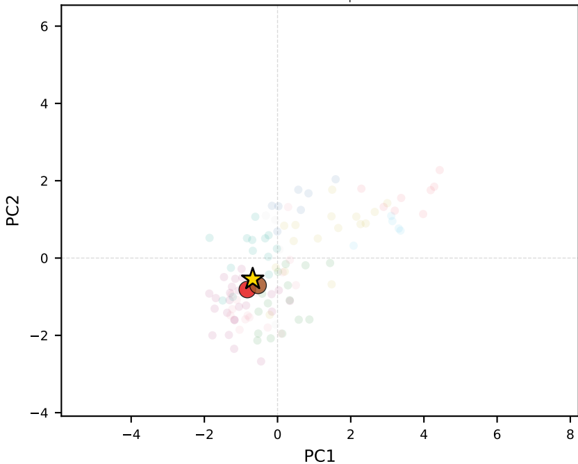
llama-3.3-70b-instruct | Kazakhstan
