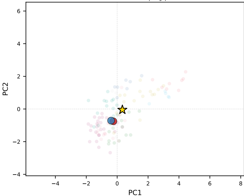
llama-3.3-70b-instruct | Singapore
