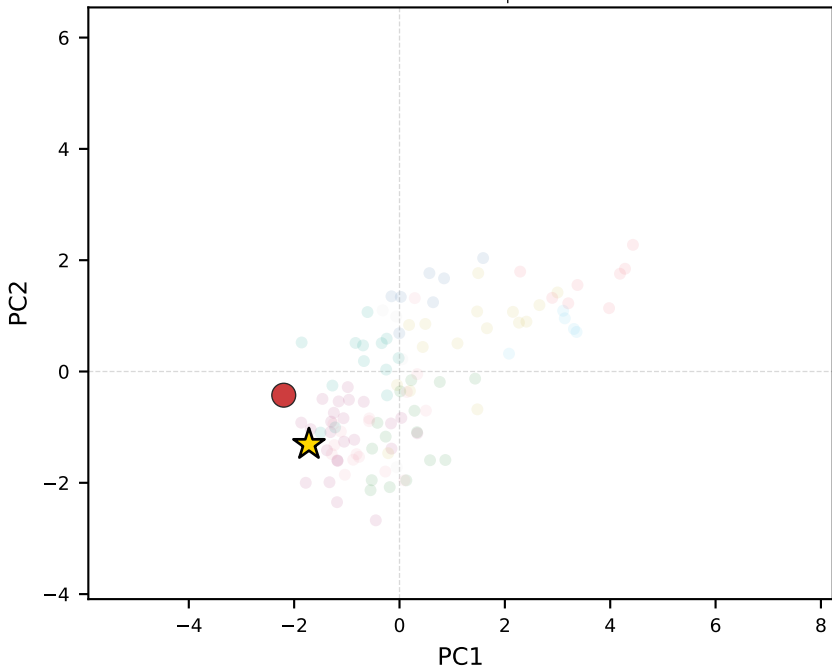
llama-3.3-70b-instruct | Zimbabwe
