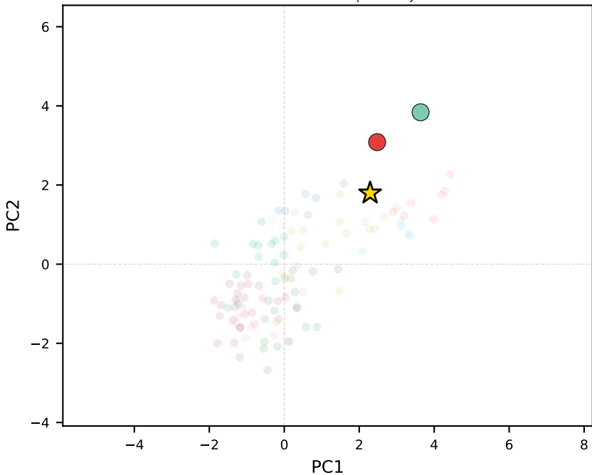
mistral-medium-3.1 | Germany
