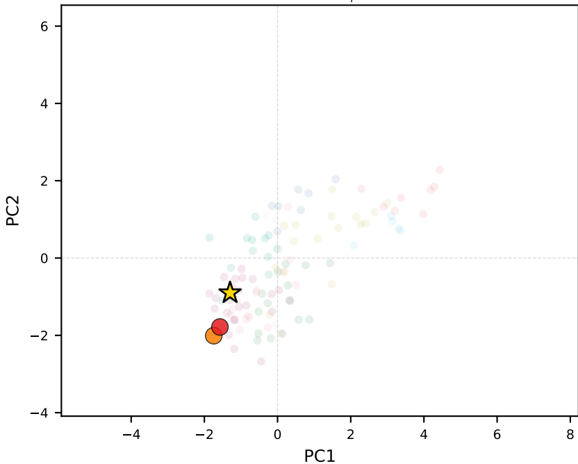
mistral-medium-3.1 | Morocco
