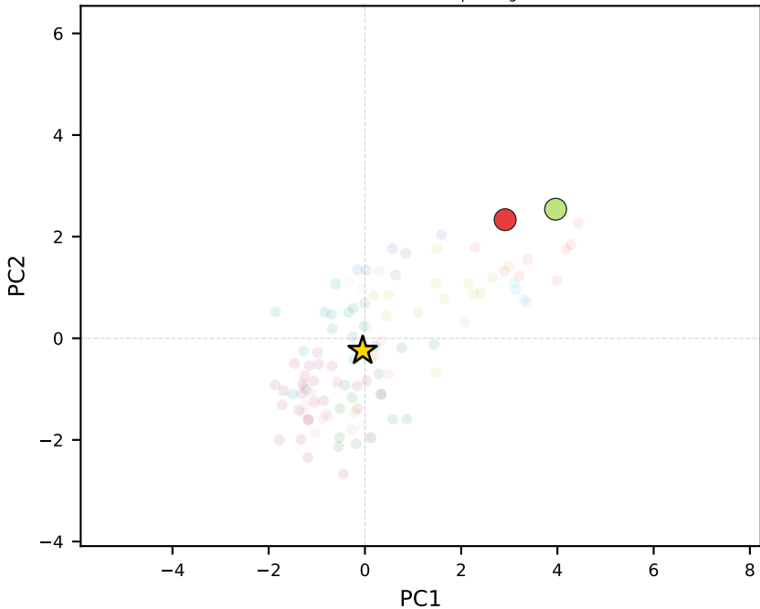
mistral-medium-3.1 | Portugal
