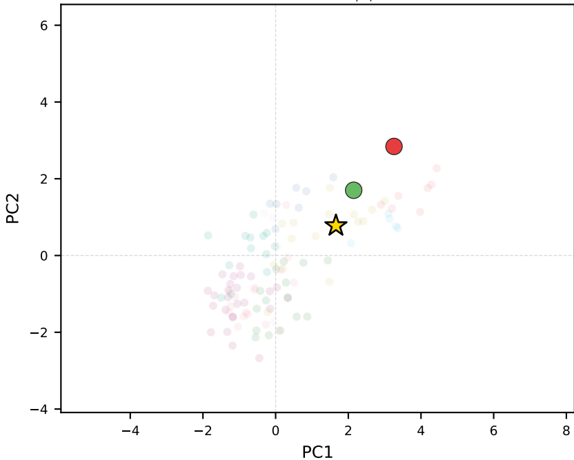
mistral-medium-3.1 | Spain
