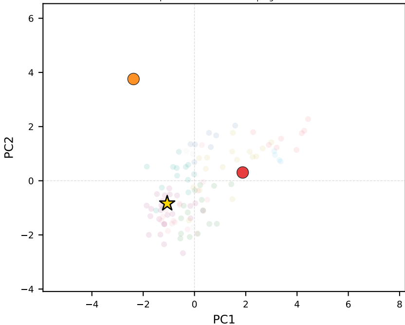
phi-3-mini-128k-instruct | Algeria
