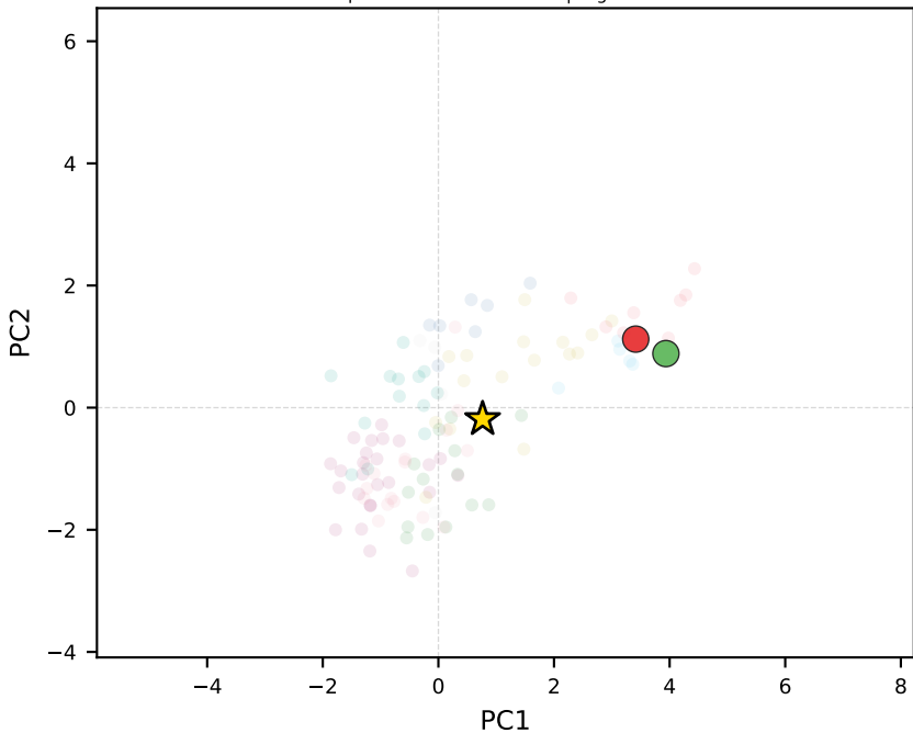
phi-3-mini-128k-instruct | Argentina
