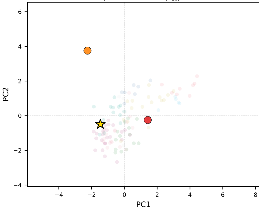
phi-3-mini-128k-instruct | Egypt
