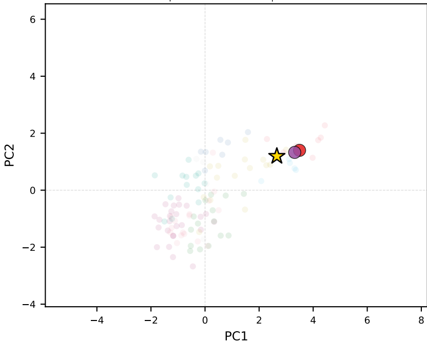
phi-3-mini-128k-instruct | France
