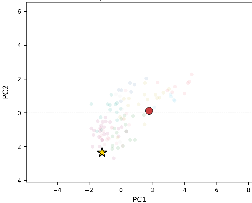
phi-3-mini-128k-instruct | Ghana
