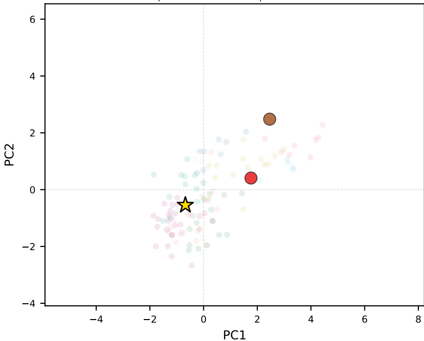
phi-3-mini-128k-instruct | Kazakhstan
