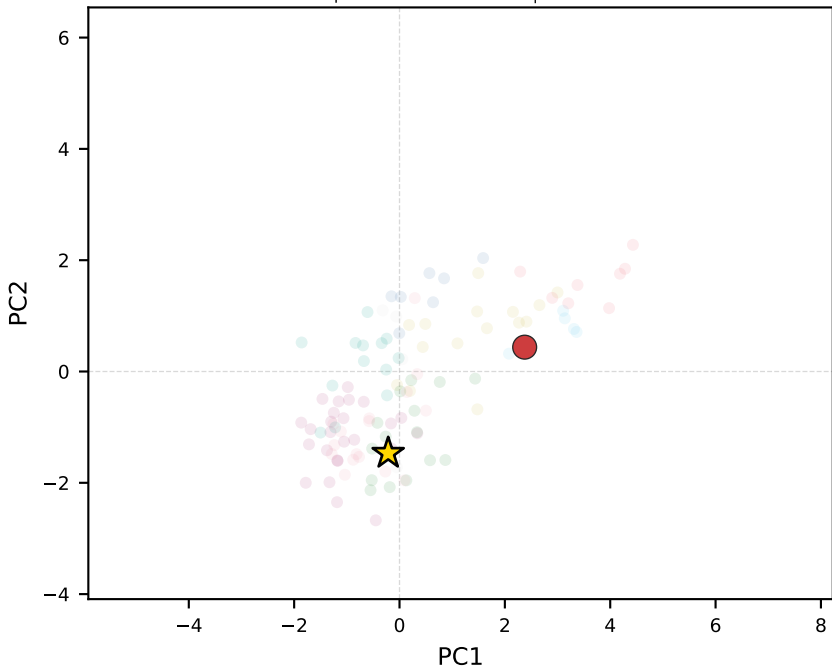
phi-3-mini-128k-instruct | Malta
