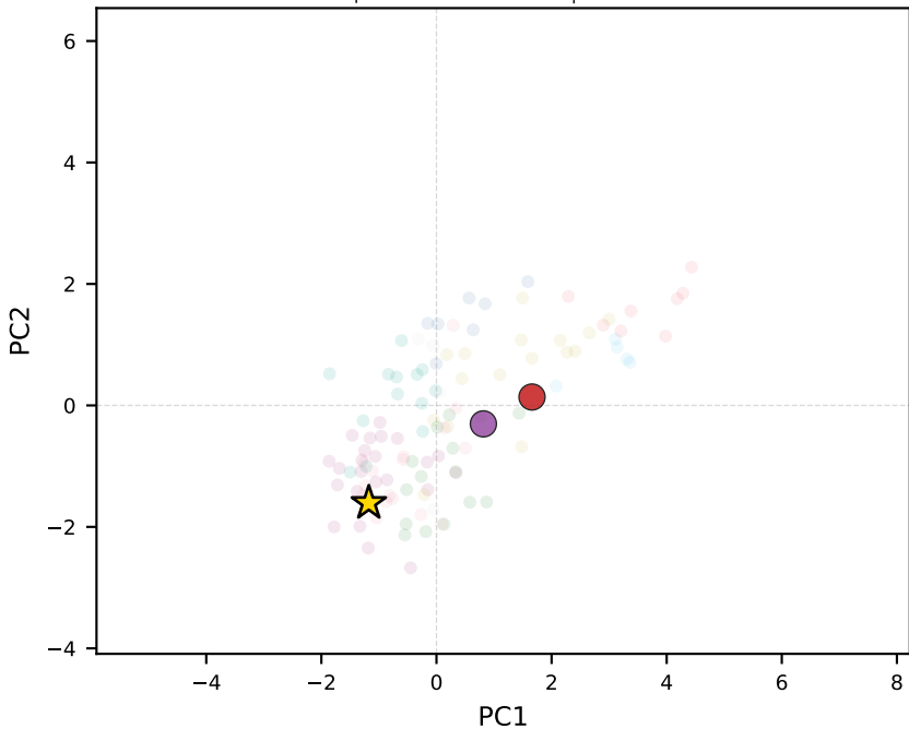
phi-3-mini-128k-instruct | Rwanda
