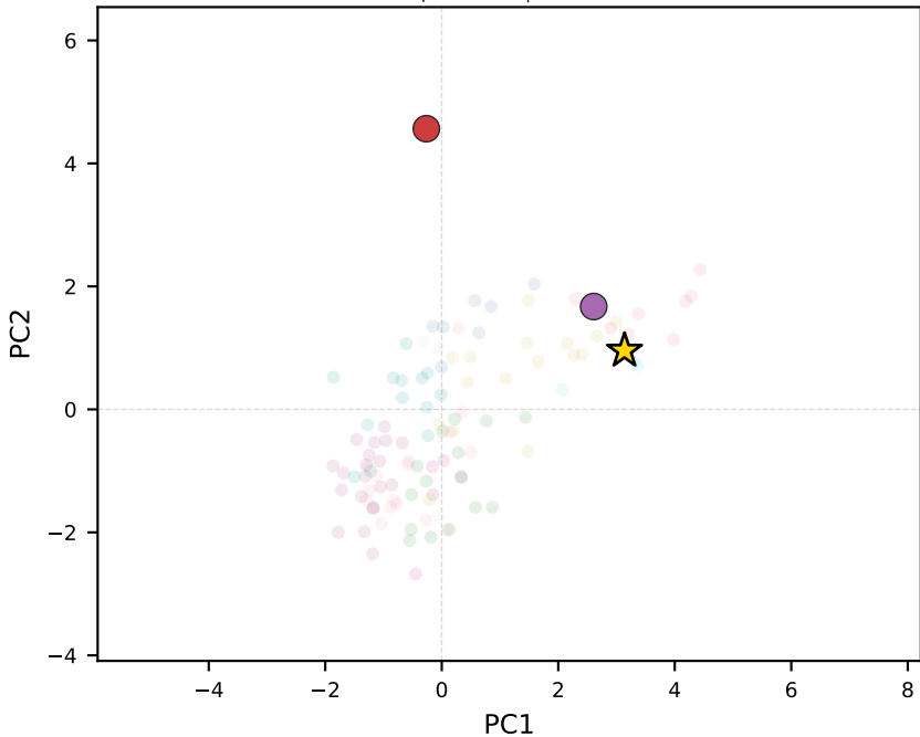
qwen3-1.7b | Canada
