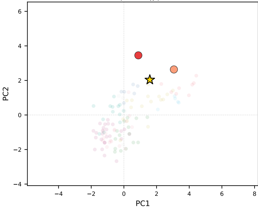
qwen3-1.7b | Japan
