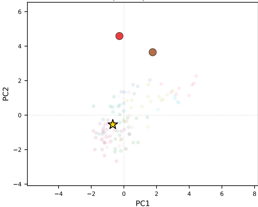
qwen3-1.7b | Kazakhstan
