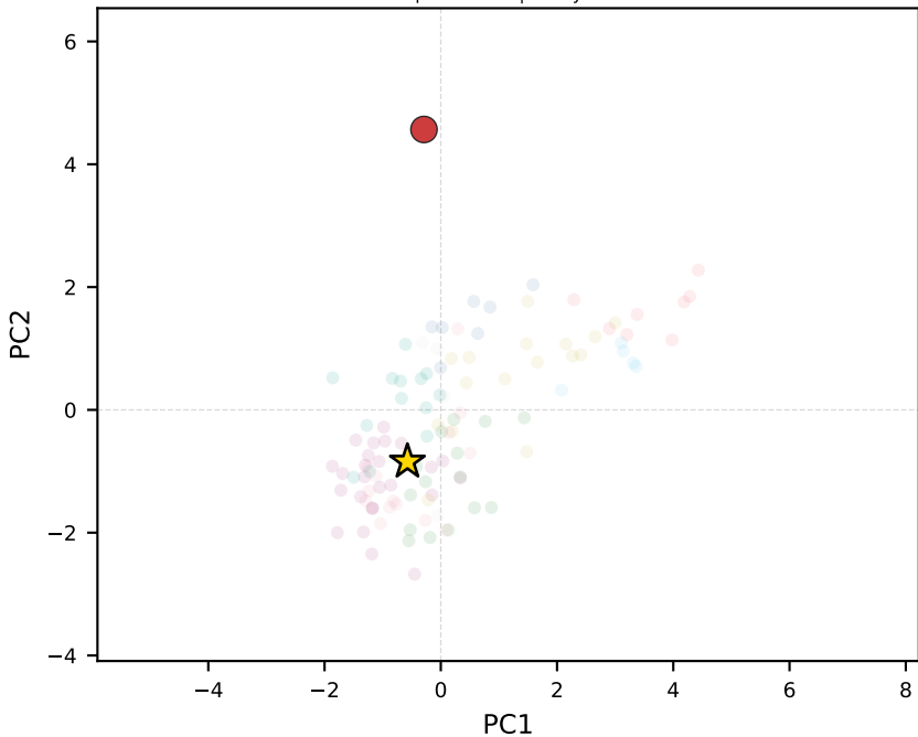
qwen3-1.7b | Malaysia
